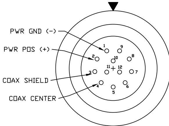
SOLDER VIEW "B"
